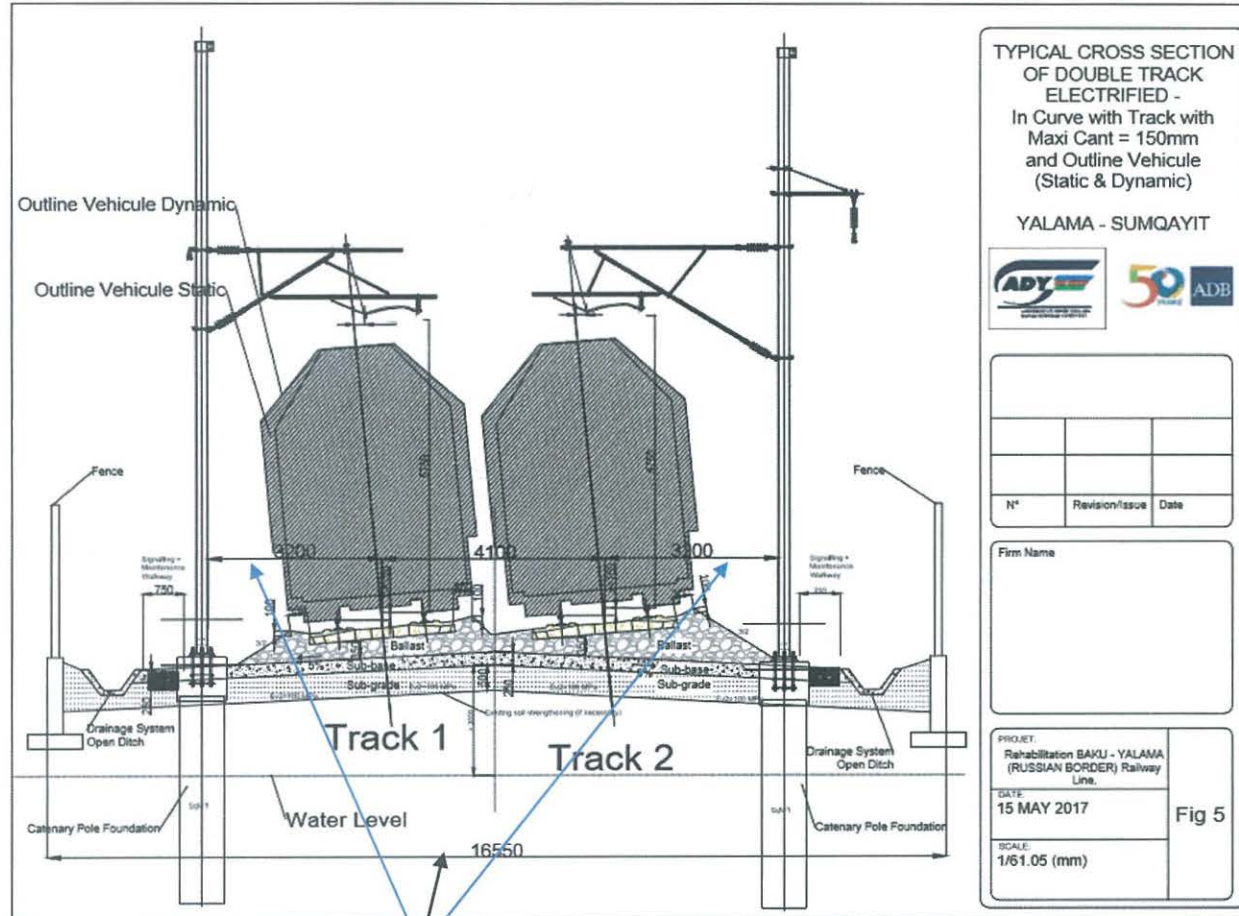
INDICATIVE CROSS SECTION LOOKING AWAY FROM BAKU
