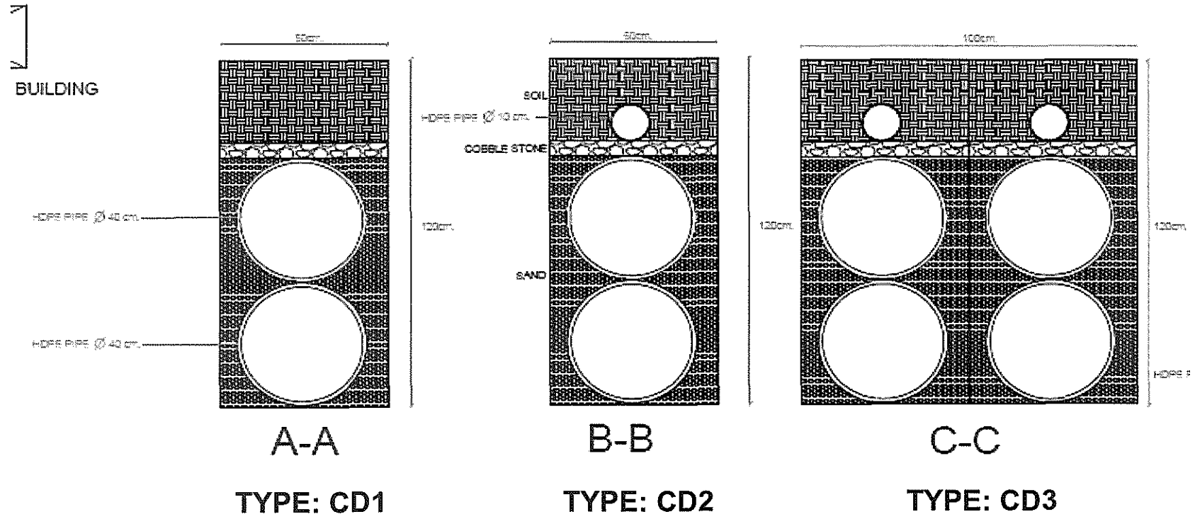
CABLE DUCTS IN STATIONS
