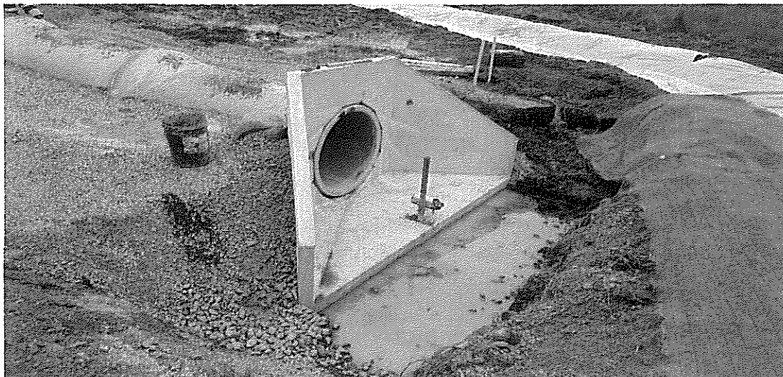
Figure 20.2 Typical Culvert End Arrangements – Pipe Culverts
