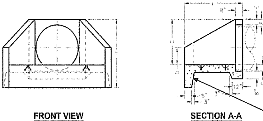
Figure 20.4 Reference Dimensions for Wing Walls, Headwall & Apron
