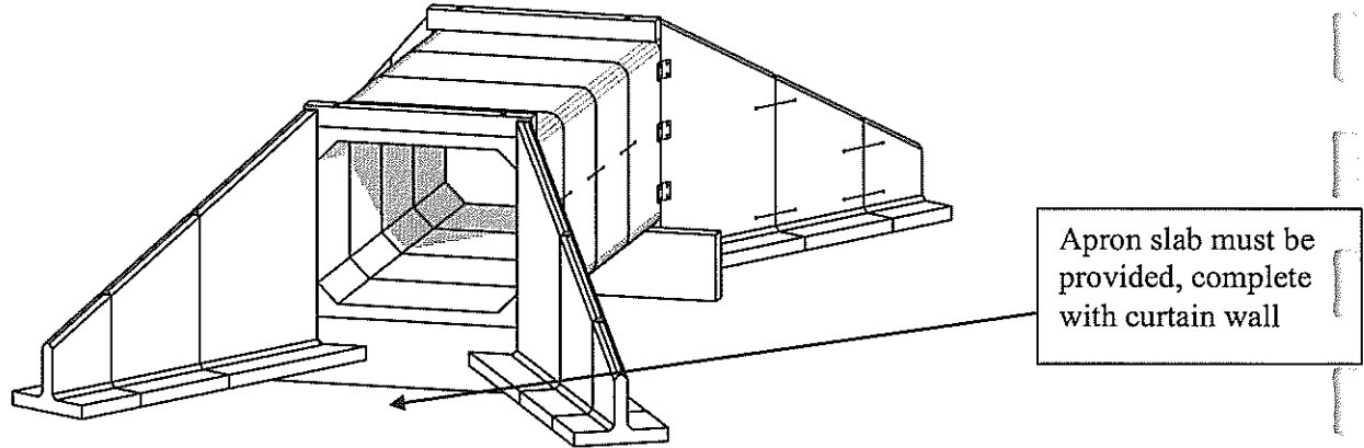
Figure 20.3 Typical Culvert End Arrangements – All Box Culverts
