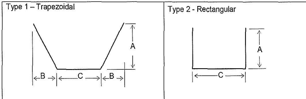
Figure 9.3 – Open Channel Types (Type 1 & Type 2)
