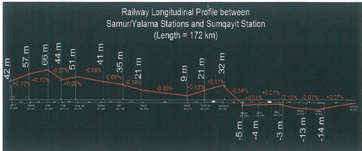
Track Elevation – Lot 1 and Lot 2
